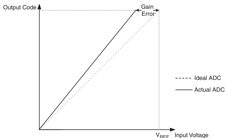
Figure 25-10. Gain Error
