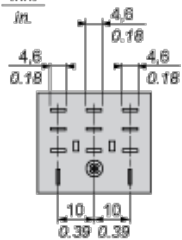
Pin Side View
