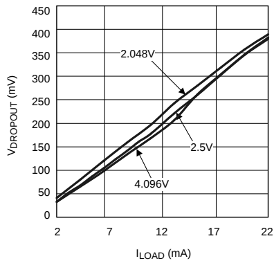
Figure 37. Dropout vs Load To 0.5% Accuracy
