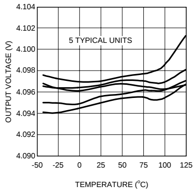
Figure 31. Output Voltage vs Temperature
