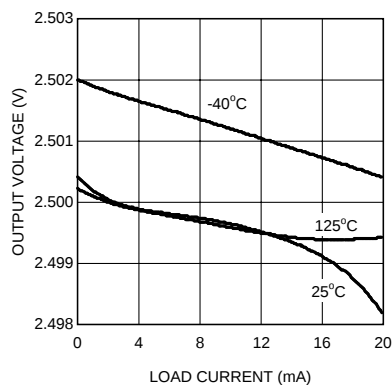
Figure 14. Load Regulation
