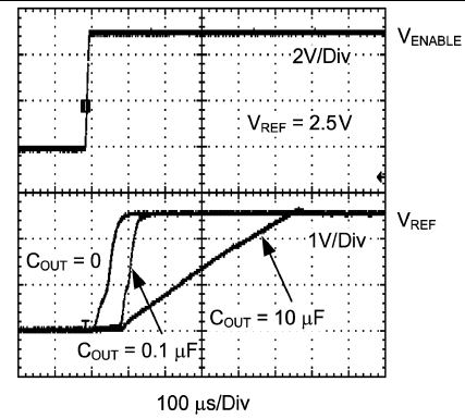
Figure 44. Turn-On Transient Response
