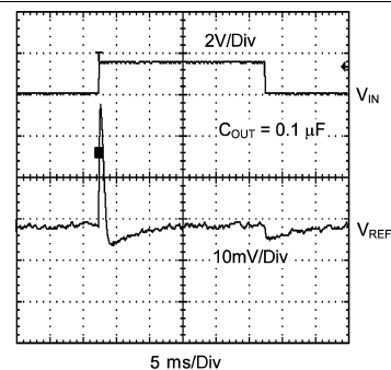
Figure 44. Turn-On Transient Response
