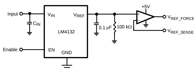
Precision Voltage Reference With Force And Sense Output
