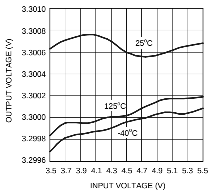
Figure 27. Line Regulation
