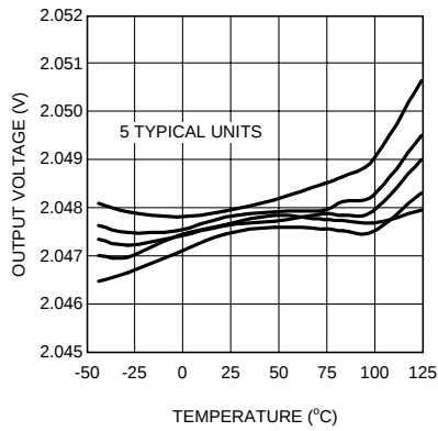
Figure 7. Output Voltage vs Temperature
