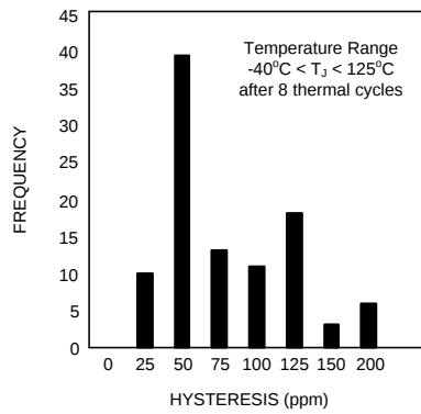
Figure 43. Typical Thermal Hysteresis
