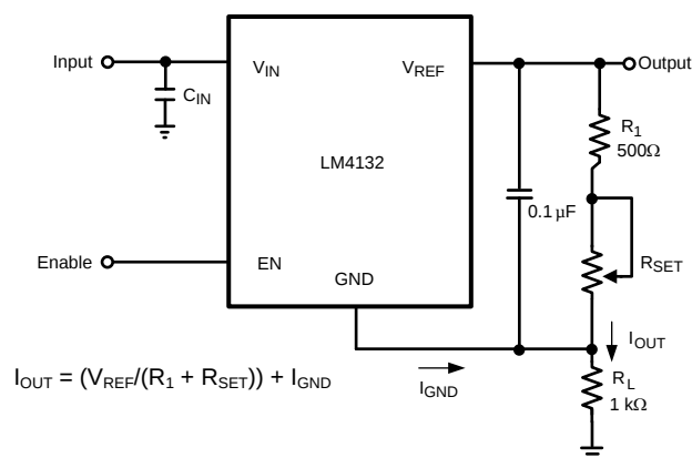
Programmable Current Source
