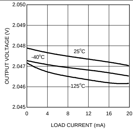
Figure 8. Load Regulation
