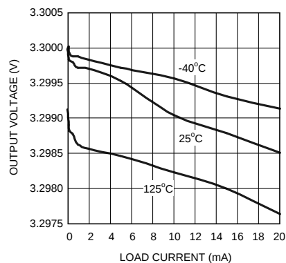
Figure 26. Load Regulation
