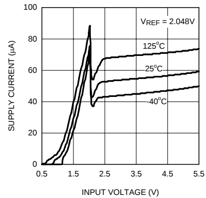
Figure 38. Supply Current vs Input Voltage
