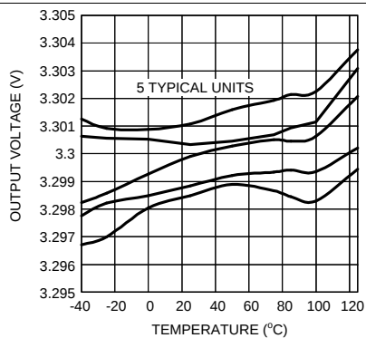
Figure 25. Output Voltage vs Temperature
