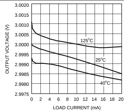
Figure 20. Load Regulation
