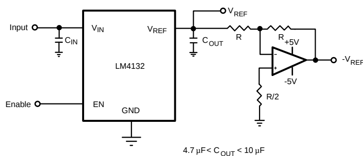
Voltage Reference With Complimentary Output
