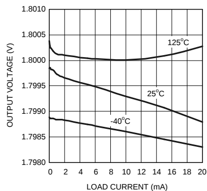
Figure 2. Load Regulation
