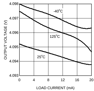
Figure 32. Load Regulation
