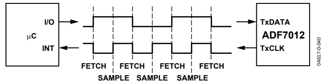
Figure 31. TxCLK/TxDATA Synchronization.
