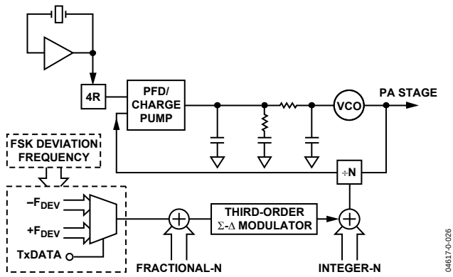
Figure 30. FSK Implementation
