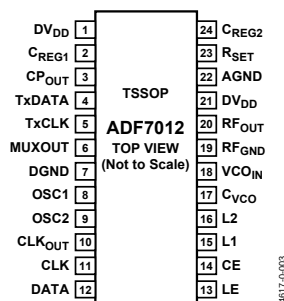
Figure 3. Pin Configuration
