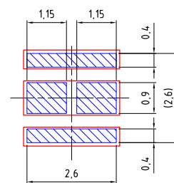
▨ solder stencil
