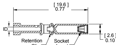
Auxiliary Socket Contacts Crimp Barrel ID
