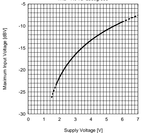
Maximum Input Voltage vs. Supply Voltage (Surround)
