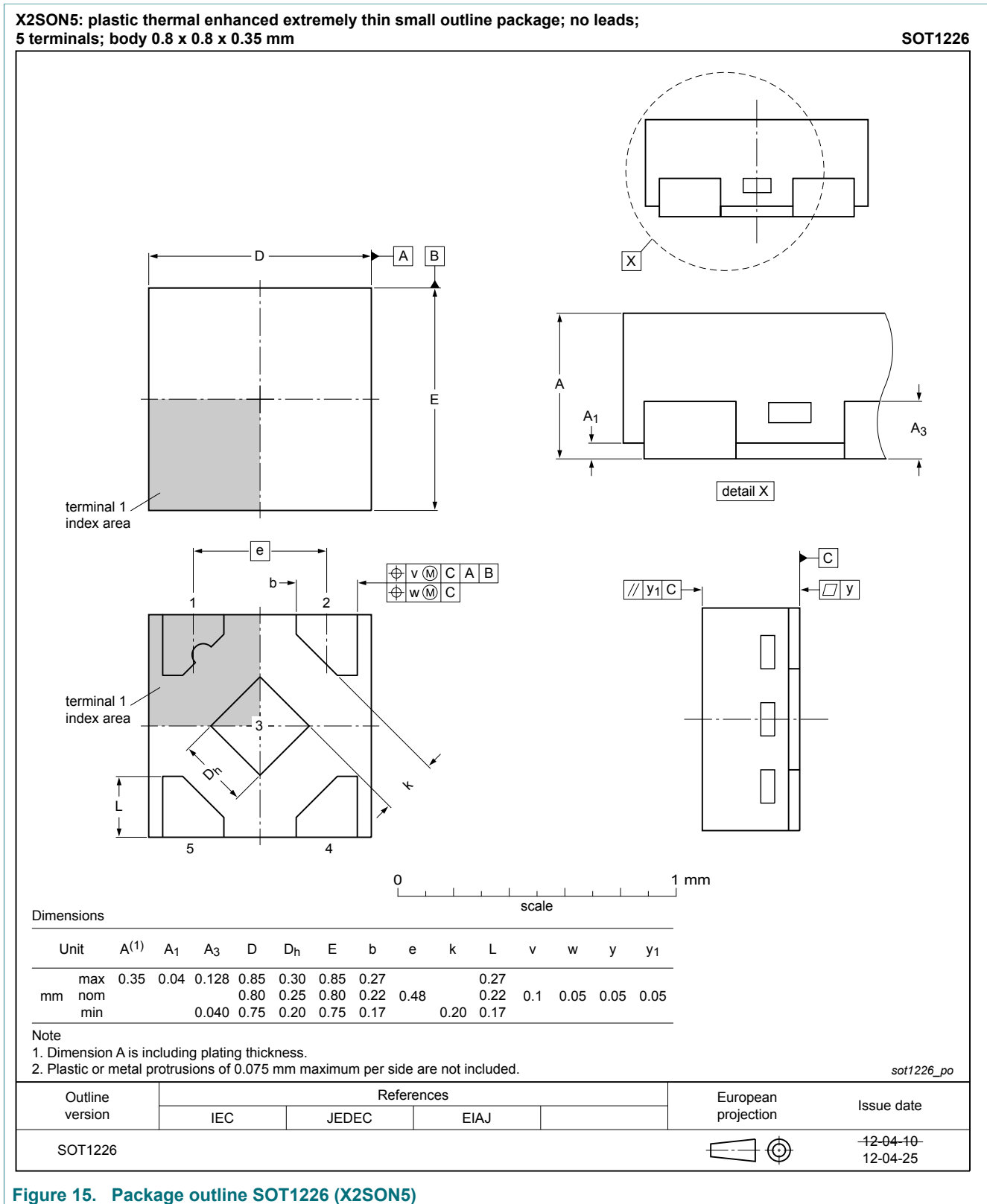
Figure 15. Package outline SOT1226 (X2SON5)
