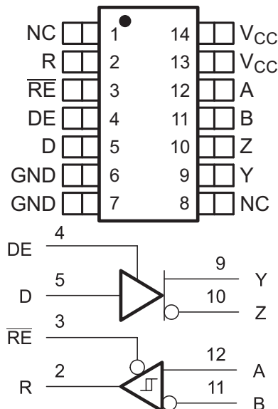
SN65HVD70, SN65HVD73, SN65HVD76 14-Pin SOIC, D Package (Top View)
