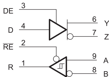
Pin Functions — MSOP-10
