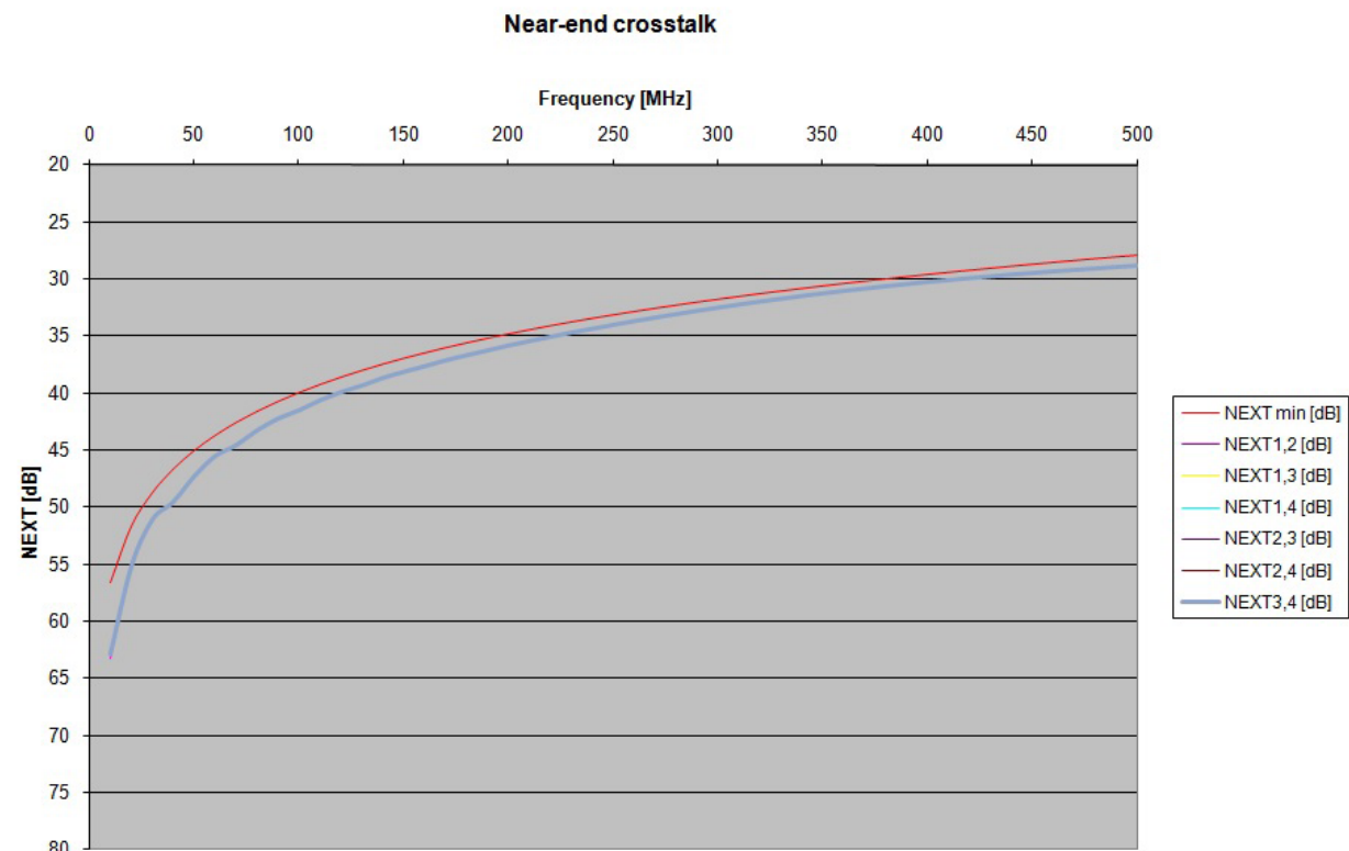
Cable assembly near-end crosstalk
