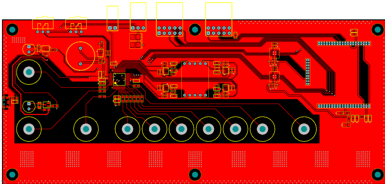
Figure 12-1 Top Layer
