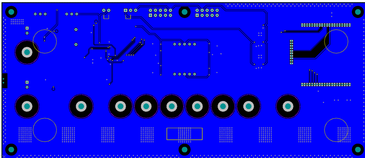
Figure 12-2 Bottom Layer
