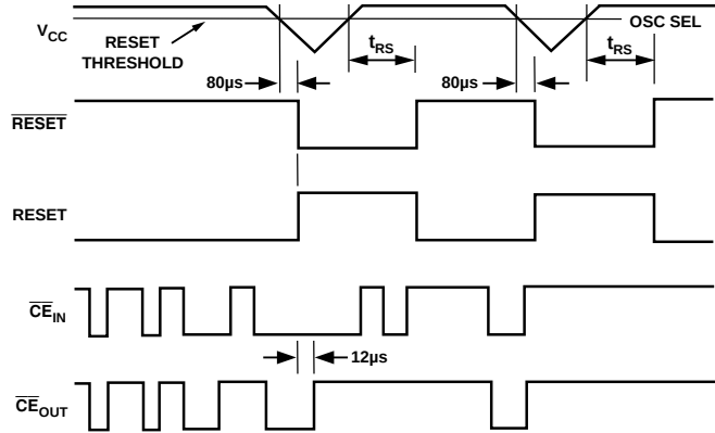
Figure 17. RESET and Chip Enable Timing
