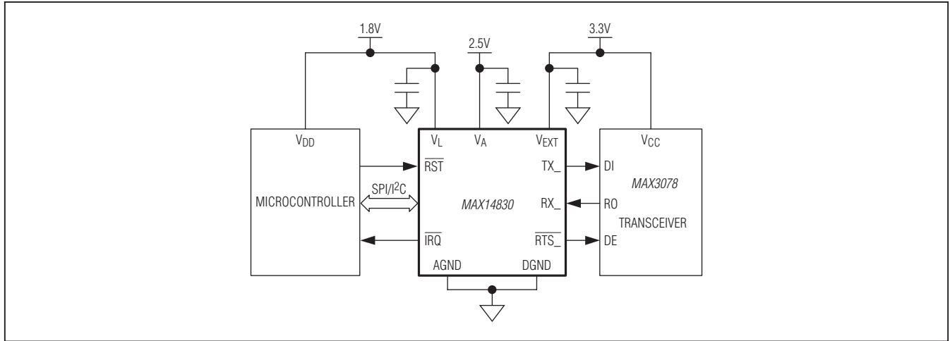
Figure 28. Logic-Level Translation
