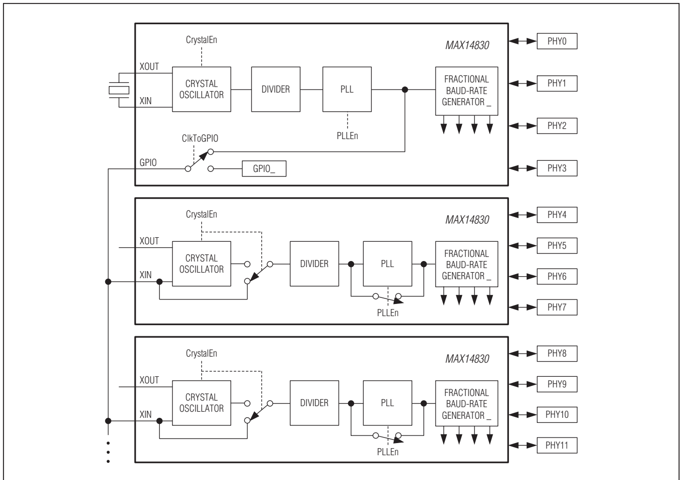
Figure 29. Interchip Synchronization
