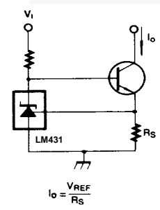
Figure 16. Constant-Current Sink
