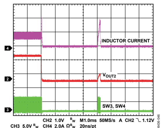
Figure 46. Current Limit Entry, Channel 2: V_{OUT} = 1.8\text{ V} , 2 A Configuration, f_{SW} = 600\text{ kHz}
