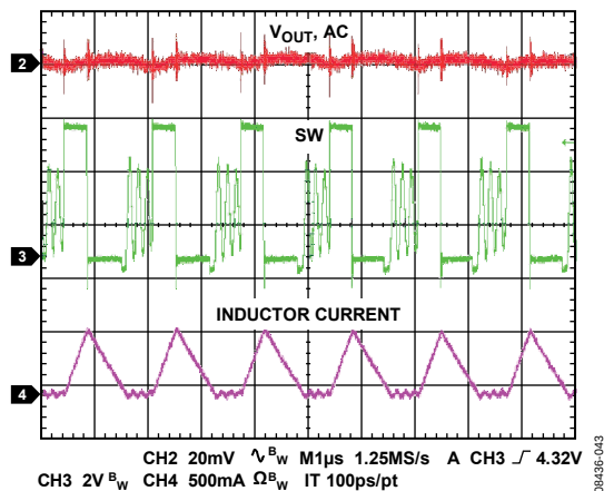
Figure 43. Pulse Skip Enabled, DCM Operation, 200 mA Load, f_{SW} = 600\text{ kHz}
