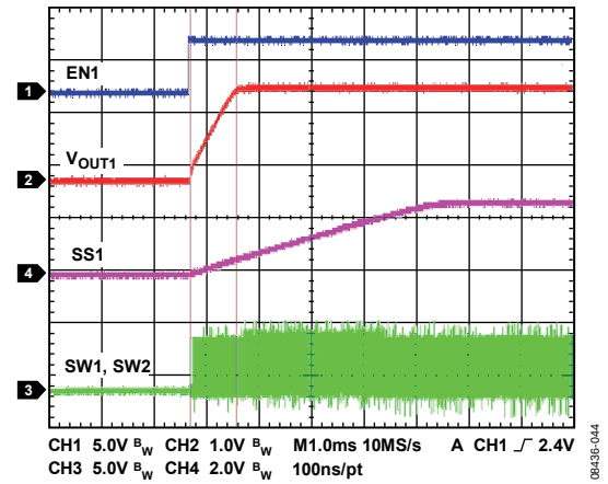
Figure 44. Soft Start, Channel 1: V_{OUT} = 1.8\text{ V} , C_{SS1} = 10\text{ nF}
