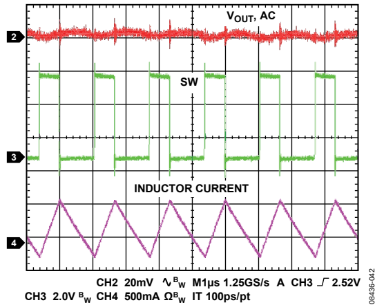
Figure 42. Forced PWM Mode, CCM Operation, 200 mA Load, f_{SW} = 600\text{ kHz}
