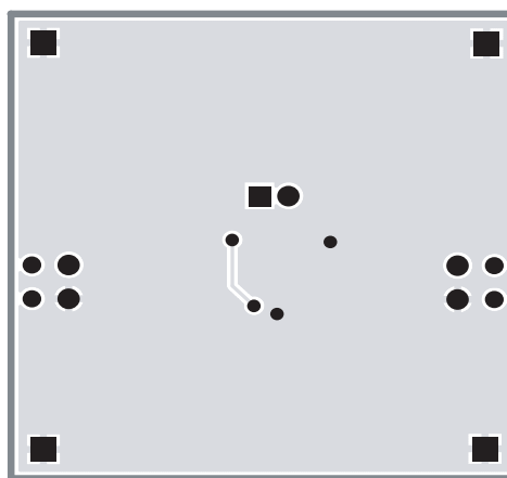
Figure 6: AAT3681A Evaluation Board Bottom Layer.
