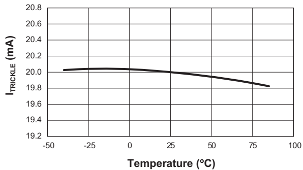
Preconditioning Charge Current vs. Temperature ( R_{SET} = 8.06k\Omega ; AAT3681A, AAT3681A-2, and AAT3681A-3 Only)
