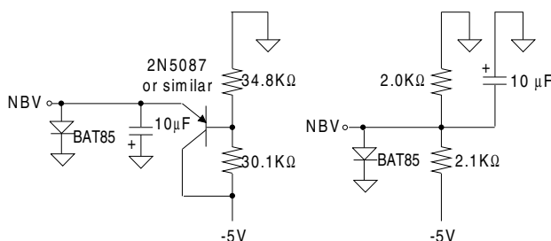
Figure 25. Alternate NBV Circuits
