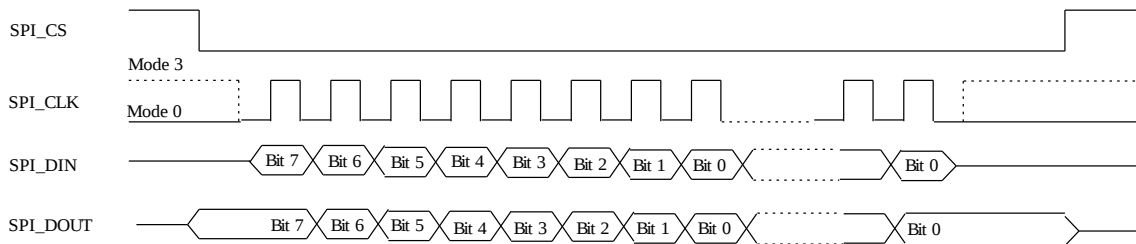
Figure 8: SPI Protocol
