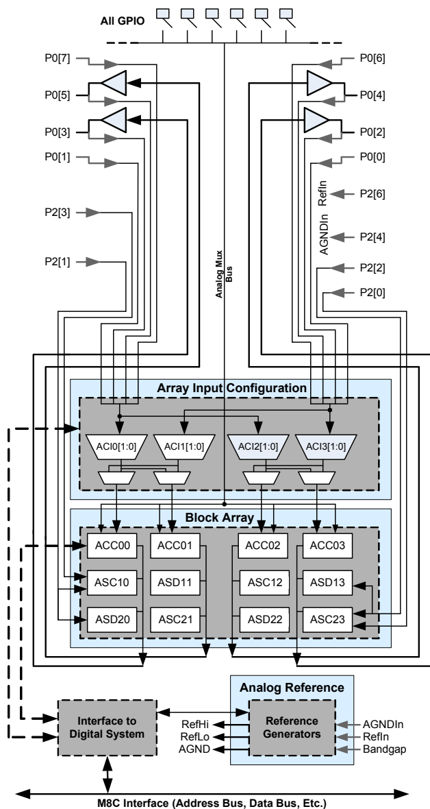
Figure 3. Analog System Block Diagram for CY8C28x43 Devices
