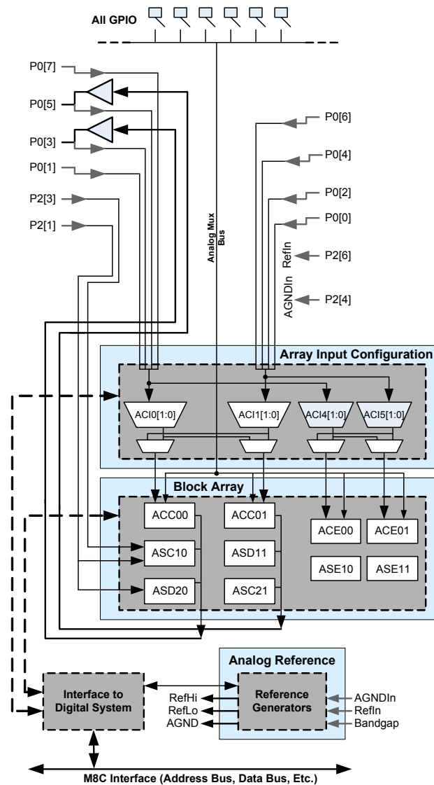
Figure 4. Analog System Block Diagram for CY8C28x33 Devices
