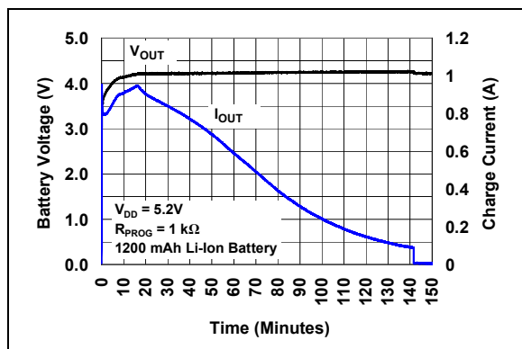
FIGURE 6-2: Typical Charge Profile (1200 mAh Li-Ion Battery).
