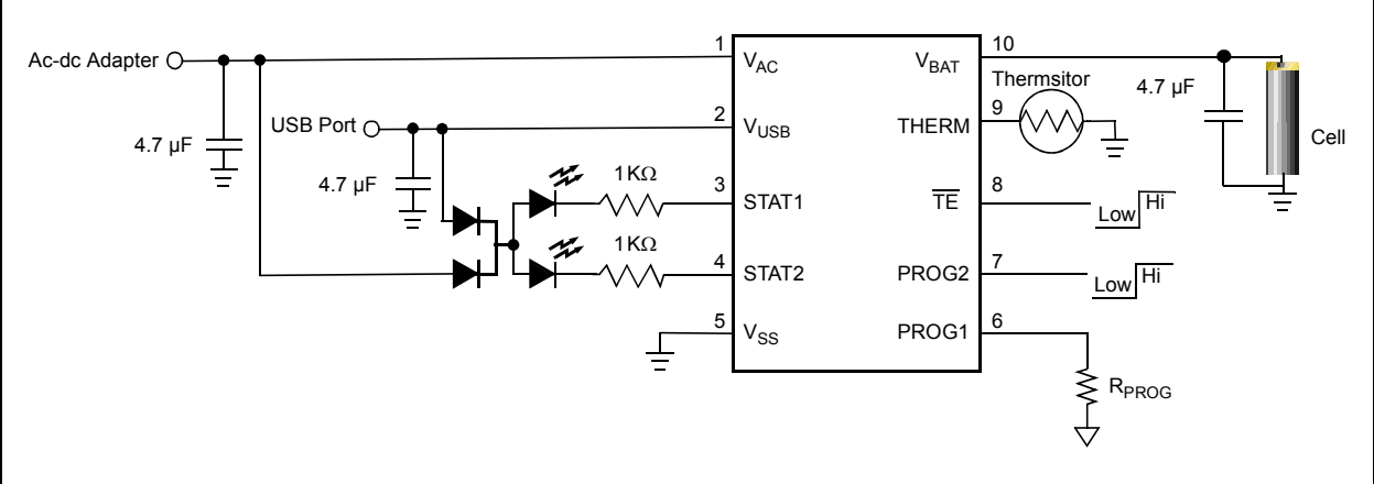
MCP73838 Typical Application
