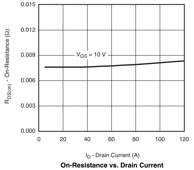
V_{GS} = 10\text{ V} On-Resistance vs. Drain Current
