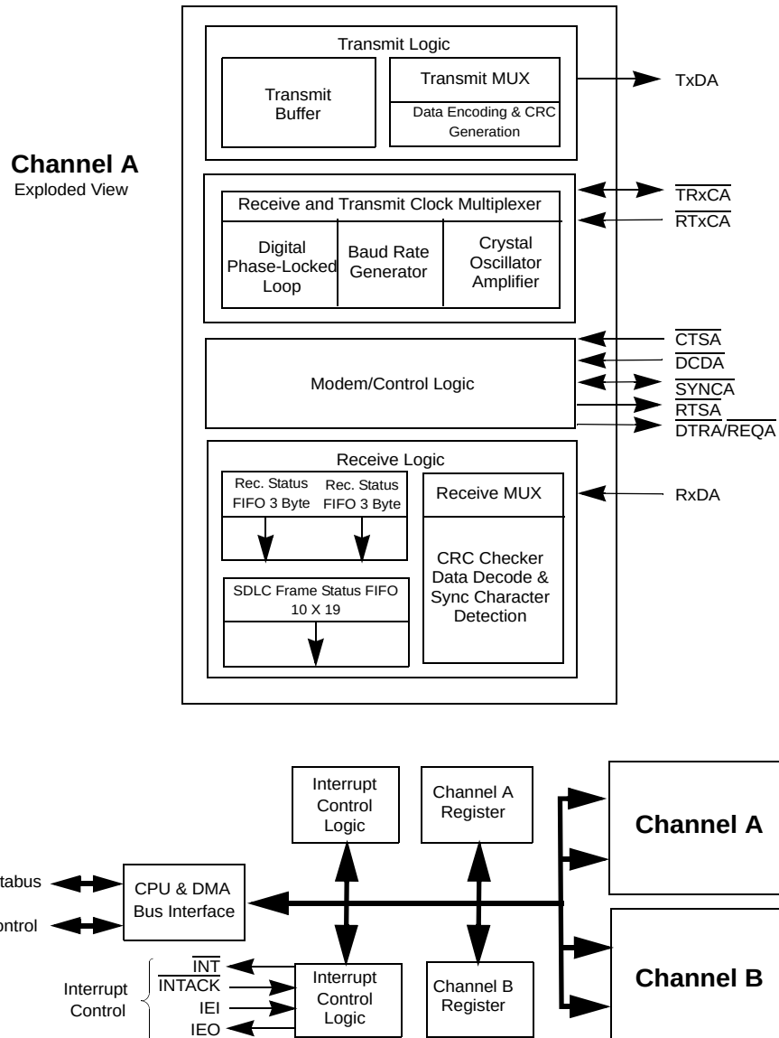
Figure 1.SCC Block Diagram
