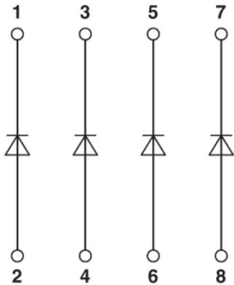
Circuit diagram
