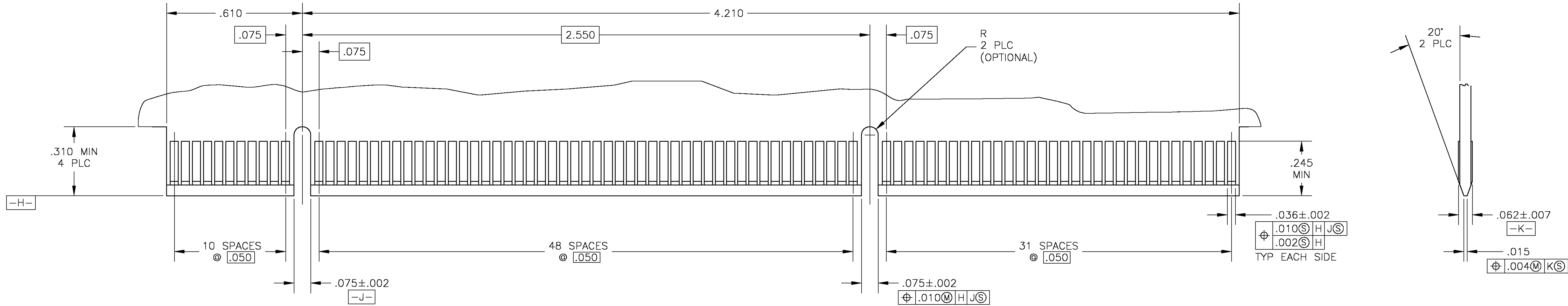
RECOMMENDED MATING BOARD EDGE CONFIGURATION
