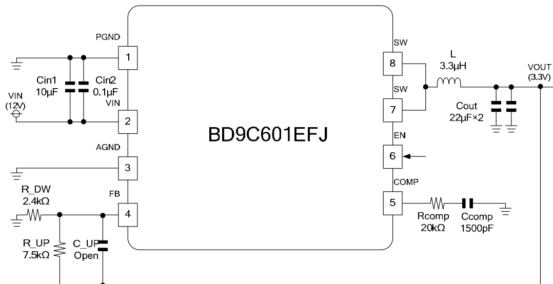
Figure 20. Application Circuit ( V_{IN}=12\text{V} , V_{OUT}=3.3\text{V} )
