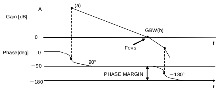
Figure 27. Bode Plot
