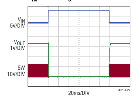
V_{IN} Overvoltage
