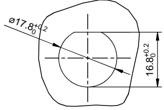
PANEL CUT OUT REFERENCE
