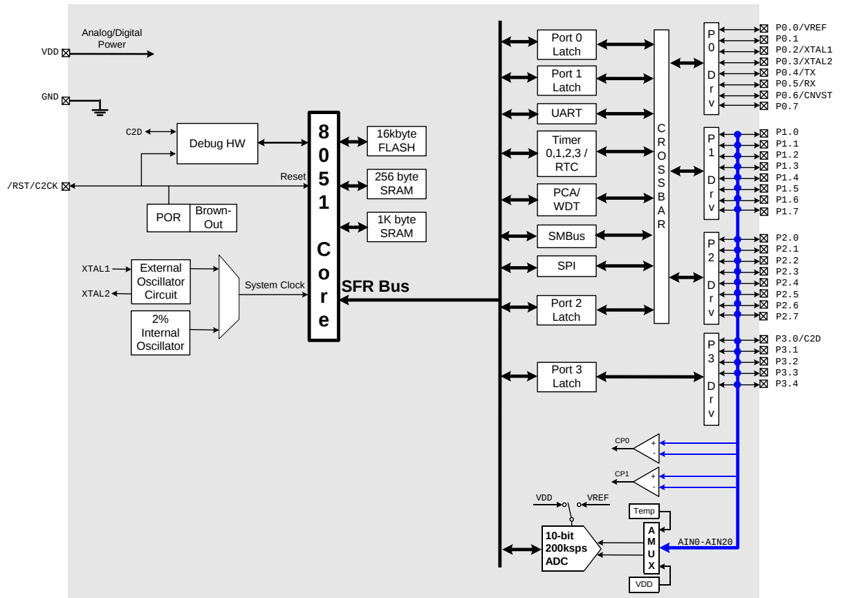
Figure 1.1. C8051F310 Block Diagram
