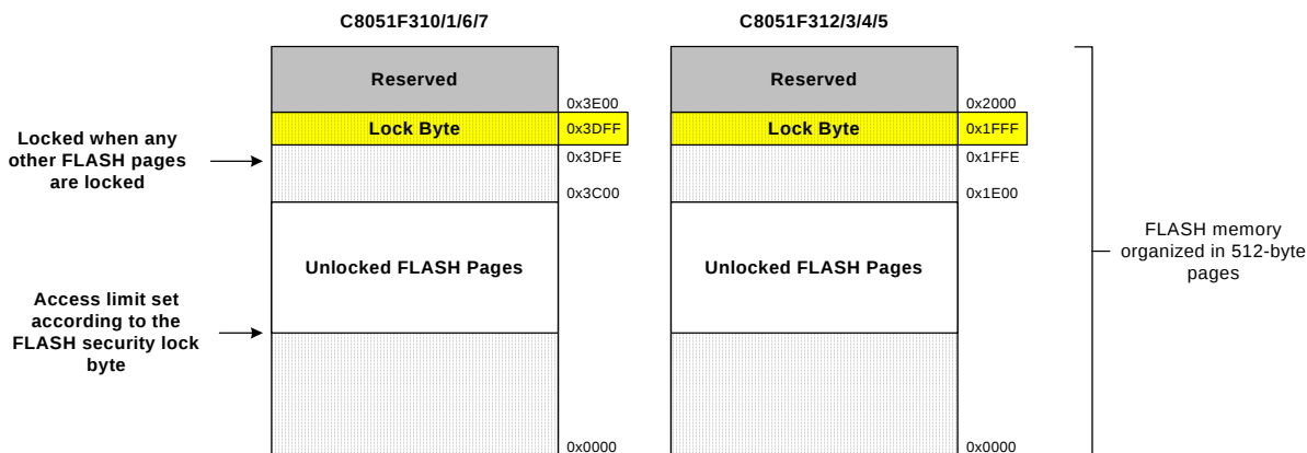
Figure 10.1. Flash Program Memory Map
