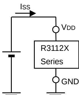
Nch Driver Output Current Test Circuit
