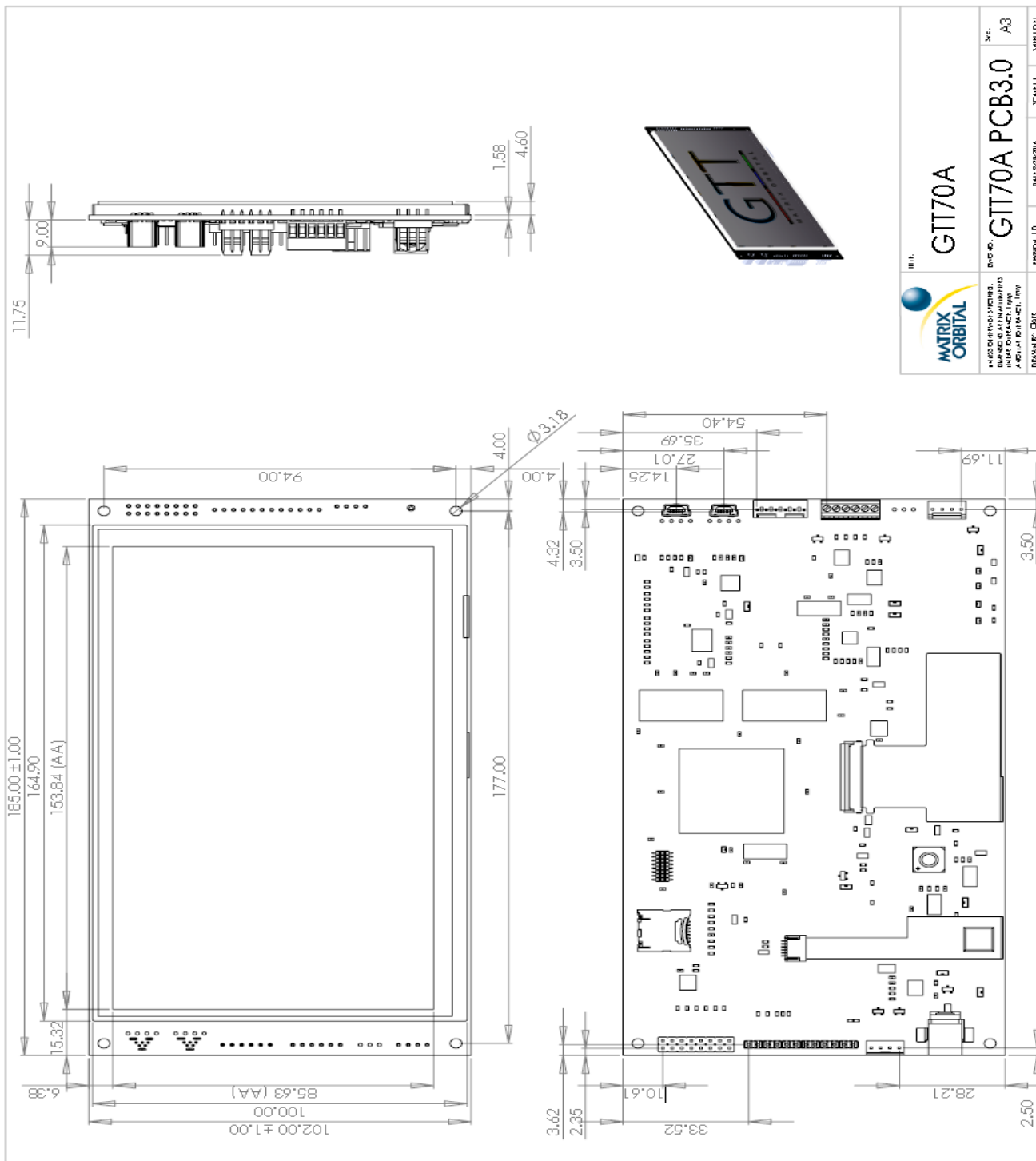
Figure 18: GTT70A Drawing
