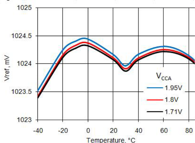
Figure 11-28. Vref vs Temperature
