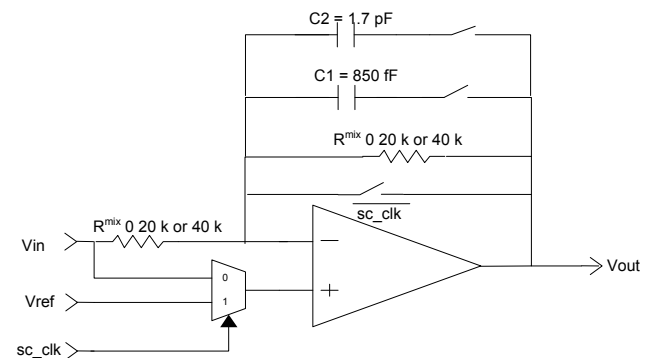
Figure 8-13. Mixer Configuration
