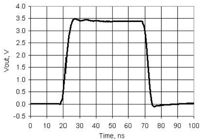
Figure 11-9. GPIO Output Rise and Fall Times, Fast Strong Mode, V_{DDIO} = 3.3\text{ V} , 25 pF Load
