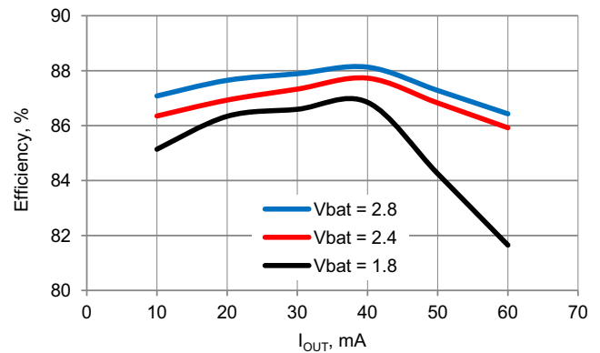
Figure 11-6. Efficiency vs I OUT V BOOST = 3.3 V, L BOOST = 22 \mu H [29]
