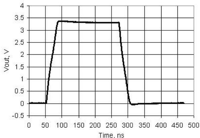
Figure 11-10. GPIO Output Rise and Fall Times, Slow Strong Mode, V_{DDIO} = 3.3 V, 25 pF Load
