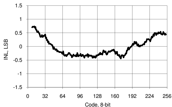
Figure 11-37. IDAC INL vs Input Code, Range = 255 \mu A, Sink Mode
