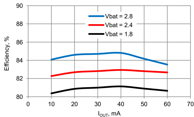
Figure 11-5. Efficiency vs I OUT V BOOST = 3.3 V, L BOOST = 10 µH [29]
