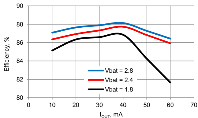
Figure 11-6. Efficiency vs I OUT V BOOST = 3.3 V, L BOOST = 22 µH [29]
