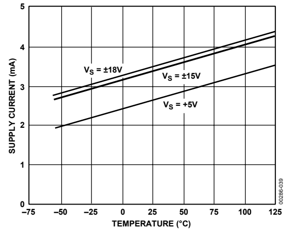
Figure 40. Supply Current vs. Temperature
