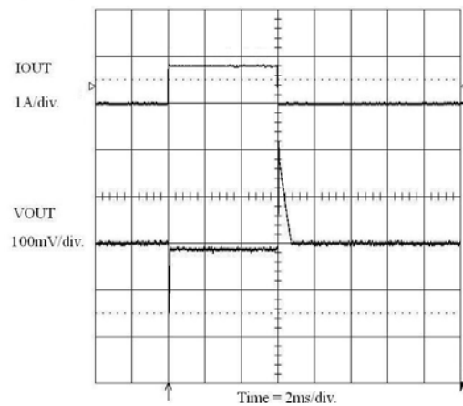
Figure 26. Load Transient Response (1 mA to 800 mA) ( V_{OUT} = 0.8\text{ V} and V_{IN} = 1.8\text{ V} )
