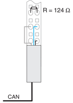
Figure 6 CAN master at the end of a CAN bus (R = 124 Ω termination resistor)
