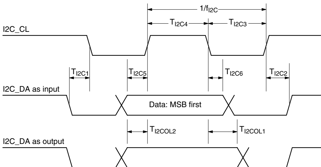
Fig. 5–2: I²C bus timing diagram
