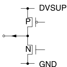
Fig. 8–12: Output pins 5, 13, 14, and 68 (I2S_DA_OUT, D_CTR_OUT0/1, TP_CO)
