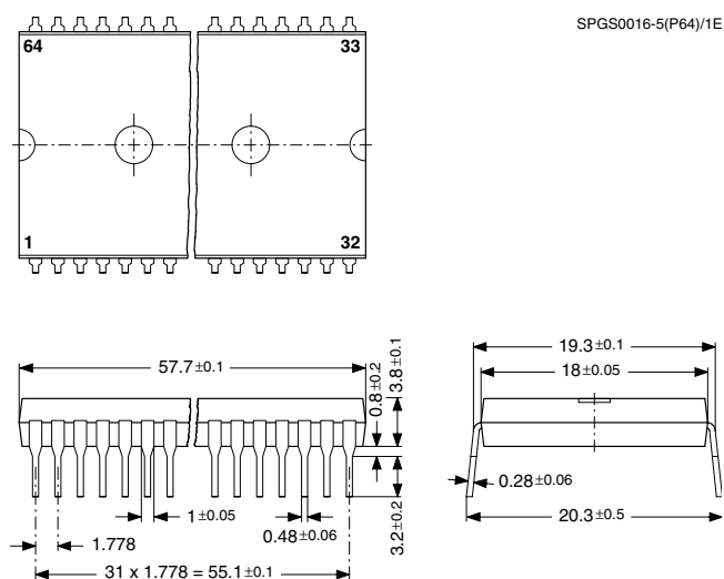
Fig. 8-2: 64-Pin Plastic Shrink Dual Inline Package (PSDIP64)
