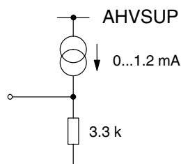
Fig. 8-22: Output Pins 56, 57 (DACM_L/R)
