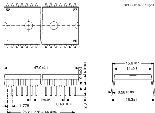
Fig. 8-3: 52-Pin Plastic Shrink Dual In Line Package (PSDIP52)
