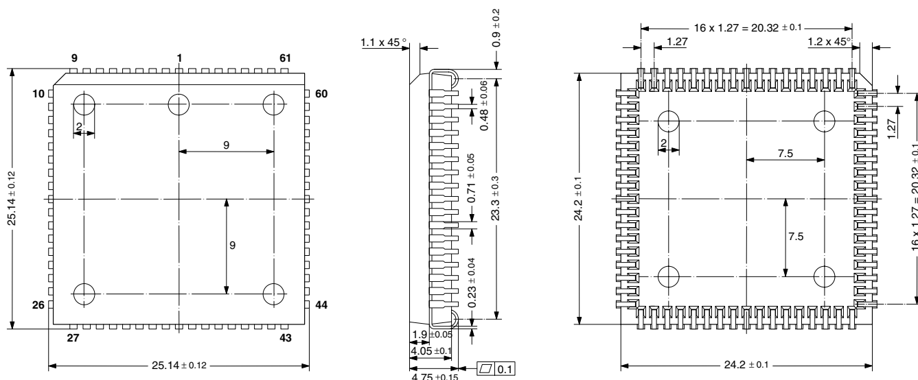
Fig. 8-1: 68-Pin Plastic Leaded Chip Carrier Package (PLCC68)
