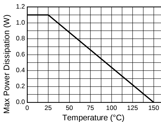
Derating Curve
