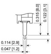
Extended PCB
