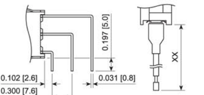
Vertical PCB Wire Leads
