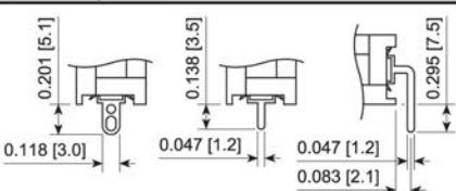
Solder Standard PCB Horizontal PCB
