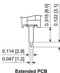
Extended PCB
