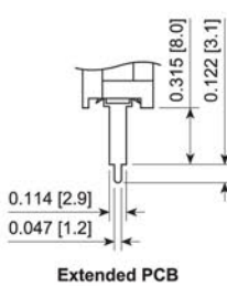
Extended PCB
