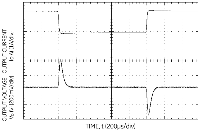
Figure 5. Transient Response to 0.1A/µS Dynamic Load Change from 50% to 75% to 50% of full load, V_{in}=48V , C_o>100\mu F .
