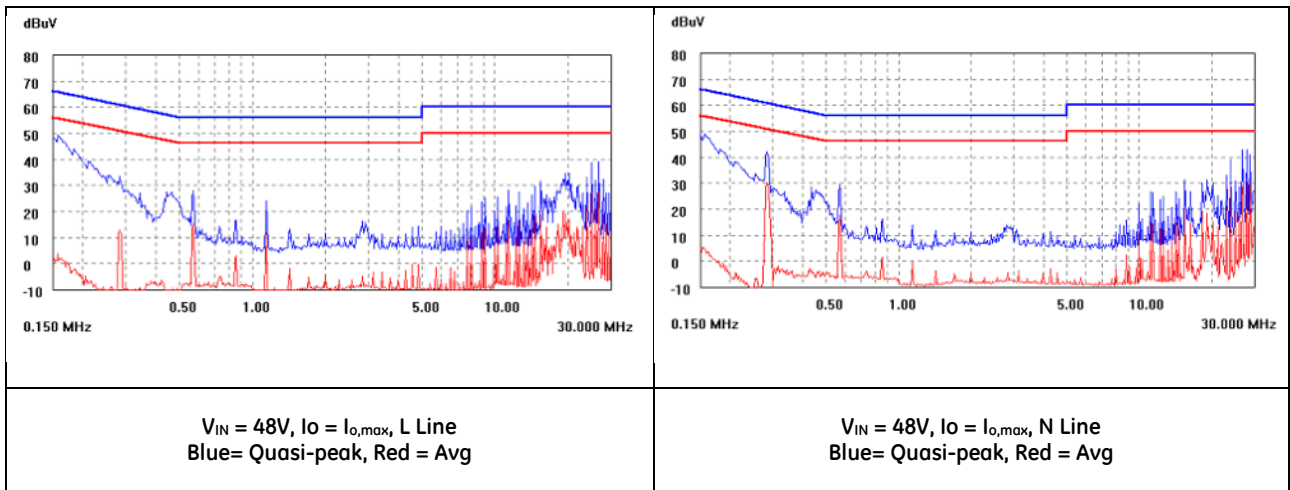
Figure 26. EMC Considerations.
