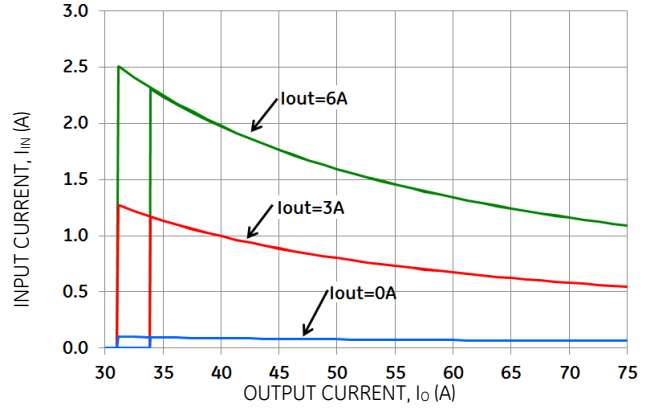
Figure 2. Input Current versus Output Current.
