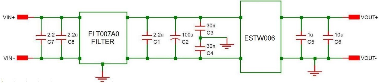
Figure 26. EMC Considerations.
