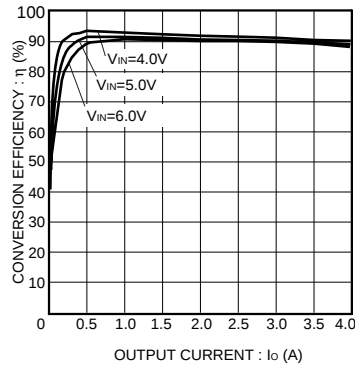
Fig.16 Conversion efficiency
