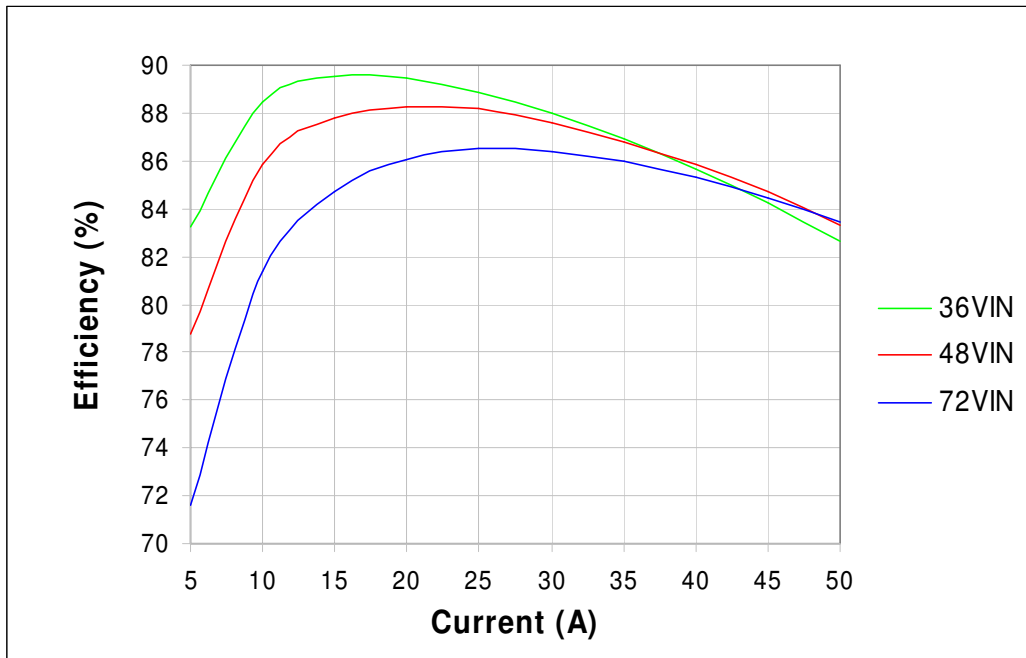
Figure 3. Efficiency (400LFM)
