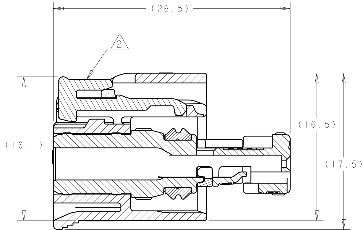
SECTION B-B
