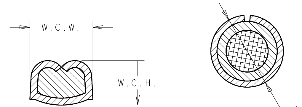
WIRE CRIMP DIMENSIONS INSULATION CRIMP DIMENSIONS
