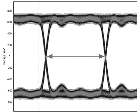
Figure 12. CML Serial Differential Output 1.25 Gbps
