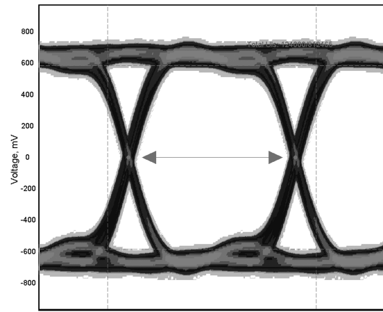
Figure 13. CML Serial Differential Output 3.125 Gbps
