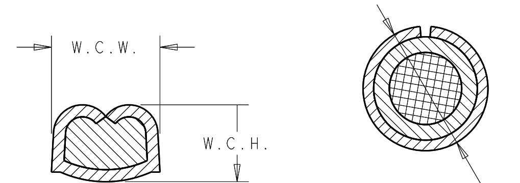
WIRE CRIMP DIMENSIONS
