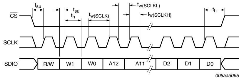
Fig 5. SPI timings
