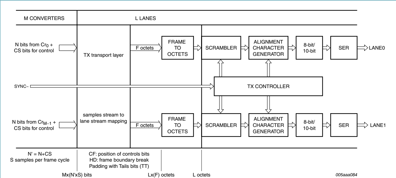
Fig 21. General overview of the JESD204A serializer
